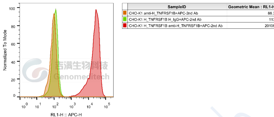
Figure 1 | H_TNFRSF1B(TNFR2) CHO-K1 Cell Line was determined by flow cytometry using Anti-H_TNFRSF1B(TNFR2) hIgG1 Antibody (Genomeditech/GM-49245AB).
